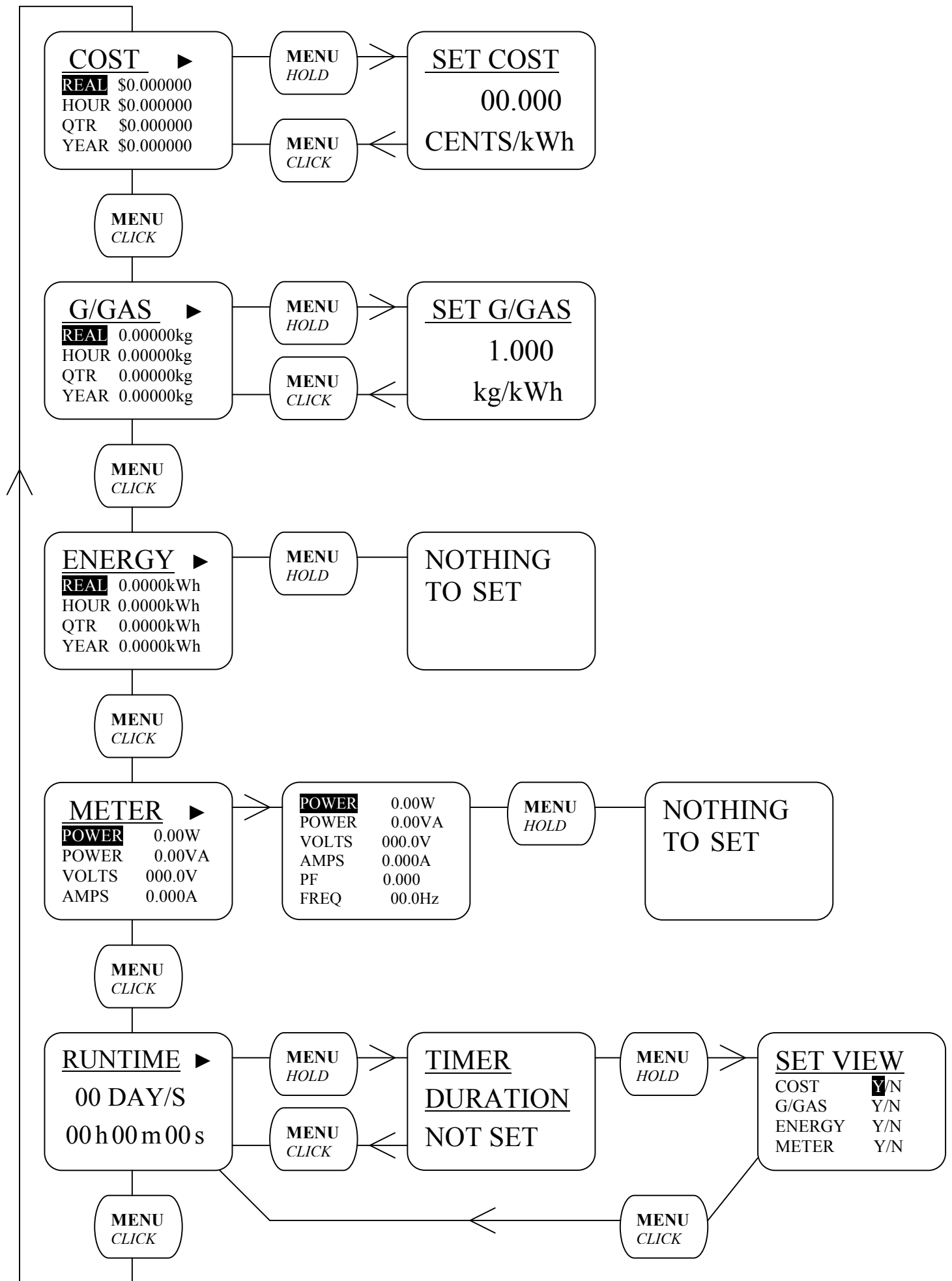
Example flow-chart of PML screen display Modes and responses to clicking or holding the Menu button. Note “click” refers to a short press of the button, “hold” refers to a longer press.
